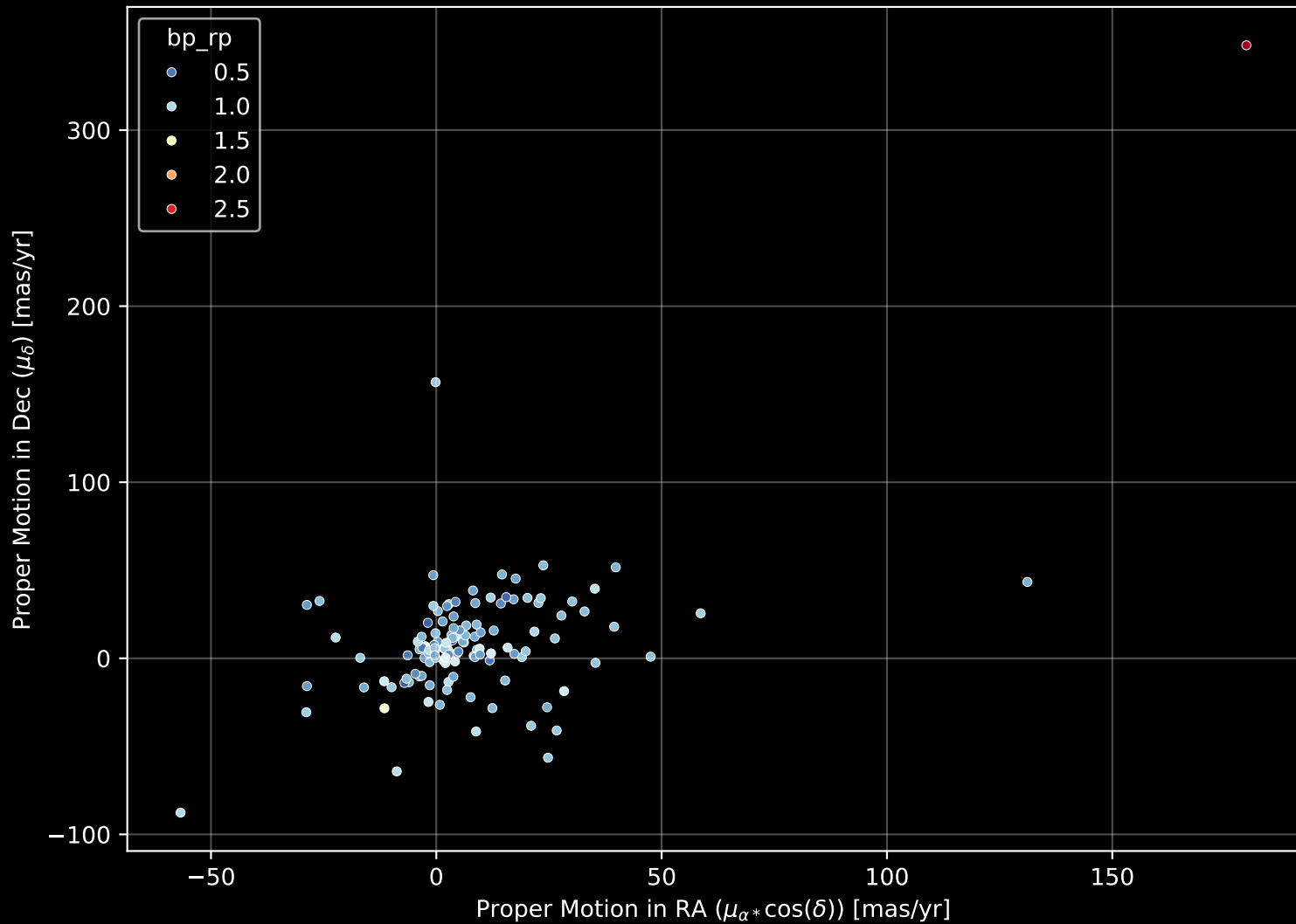
GALAH DR4 Field: [7180] Proper Motion Diagram (n= 126)
