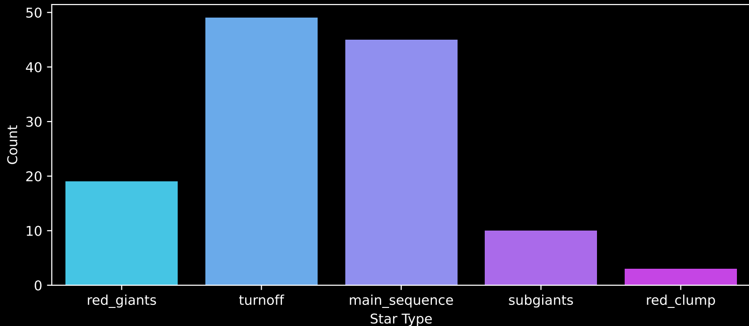
GALAH DR4 Field: [7180] Count plot of Star Type
