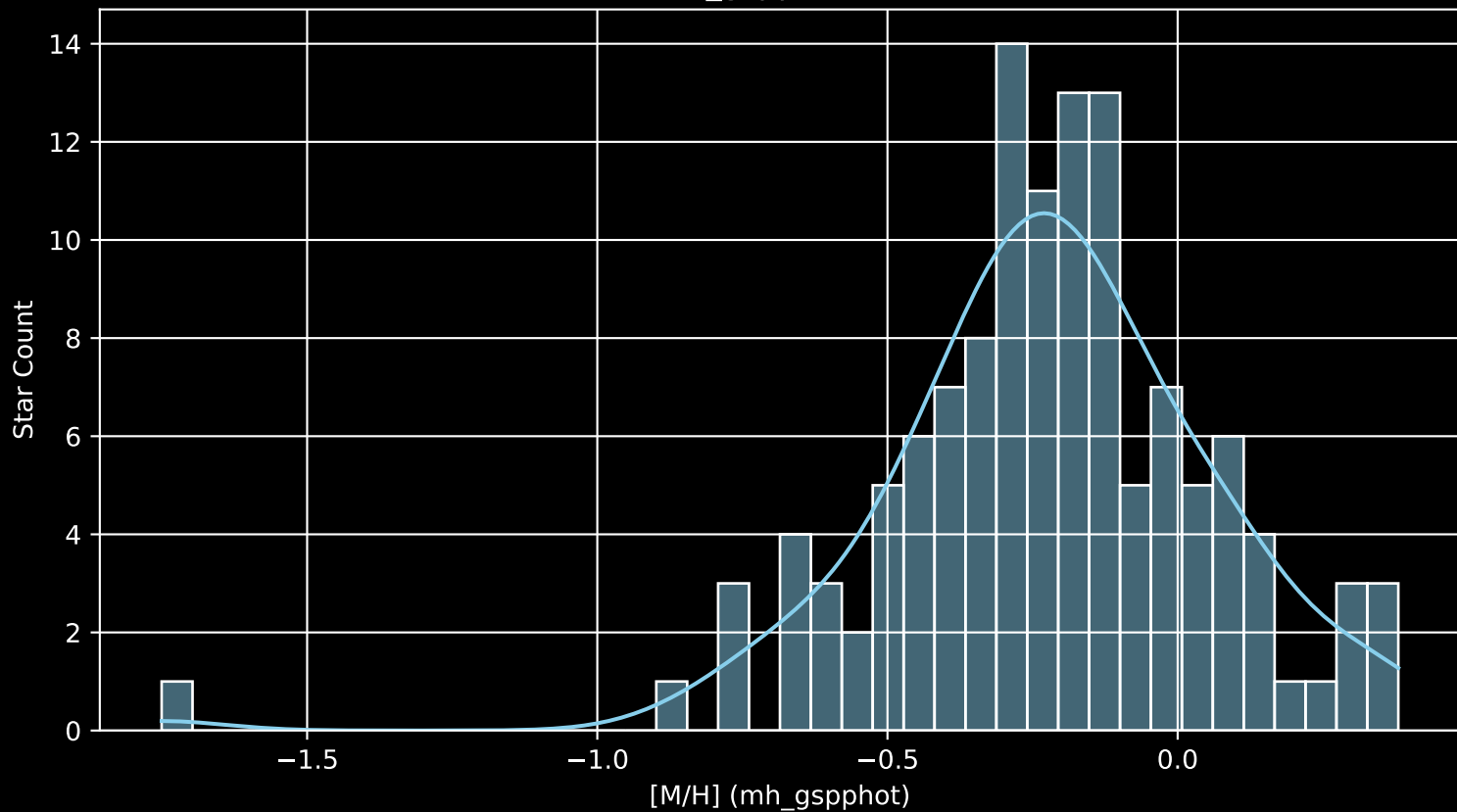
GALAH DR4 Field: [7180] [M/H] (mh_gspphot) (n= 126)
