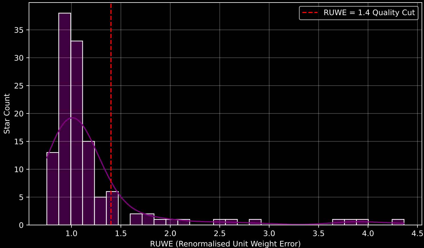
GALAH DR4 Field [7180] RUWE Distribution (n= 124)
