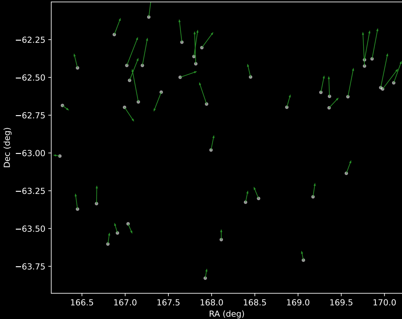
GALAH DR4 Cluster 4 Proper Motion Vectors (n=42)
